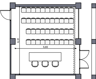
HERA Meeting Room (Lobby) 44.1 m 2 h= 2.85m
